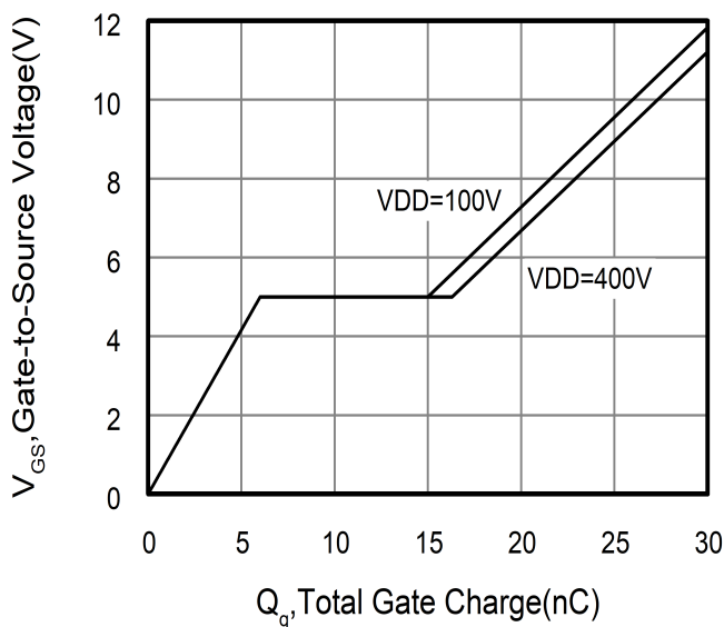
Figure 5. Gate Charge
