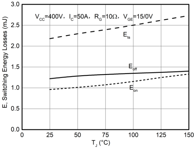
Figure 15. E_{on}, E_{off} as a function of T_j
