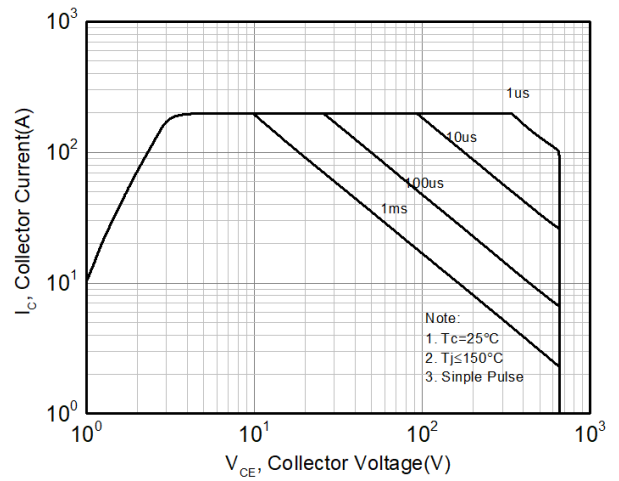
Figure 16. FBSOA
