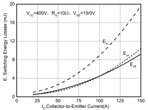
Figure 12. E_{on} , E_{off} as a function of I_C ( T_f=150^\circ C )
